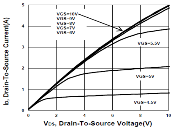
Output Characteristics
