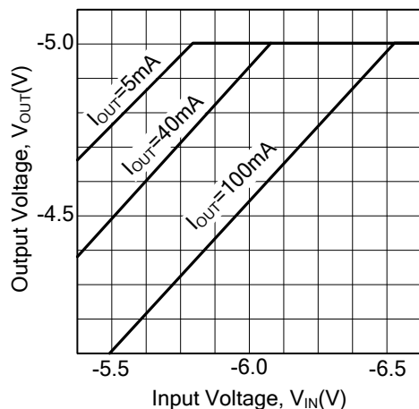
79L05 Dropout Characteristics ( T_J=25^\circ\text{C} )
