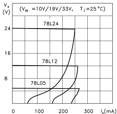
Figure 2 : Load Characteristics
