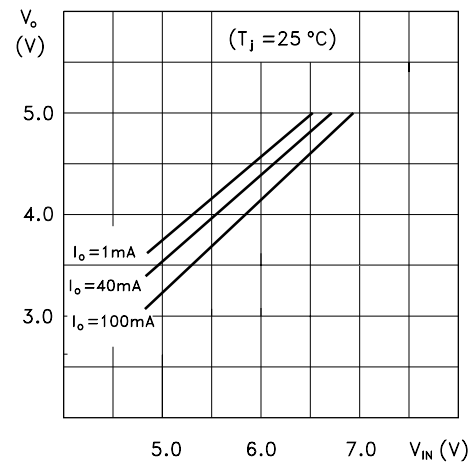
Figure 8 : Dropout Characteristics
