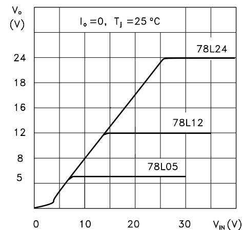
Figure 6 : Output Characteristics
