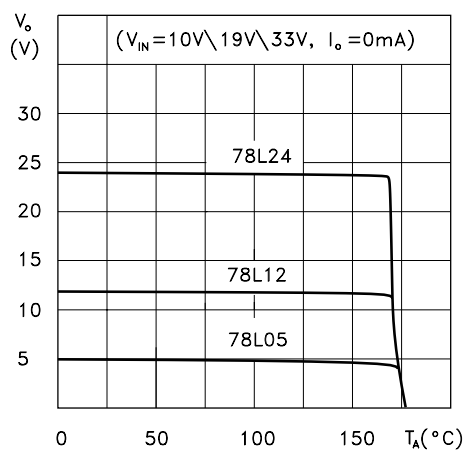
Figure 3 : Thermal Shutdown
