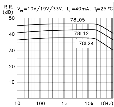
Figure 7 : Ripple Rejection
