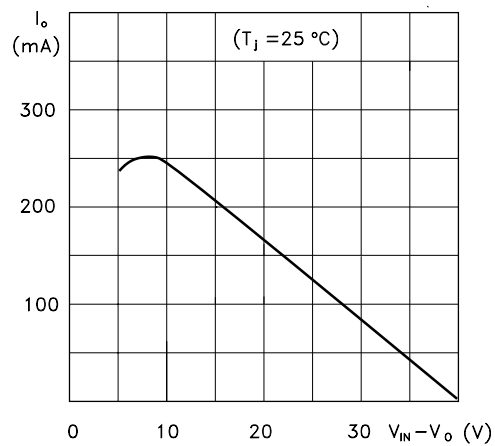
Figure 9 : Short Circuit Output Current
