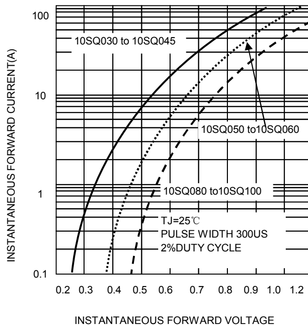
FIG.4-TYPICAL FORWARD CHARACTERISTICS
