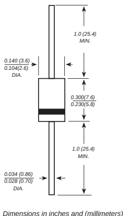
DO-15
