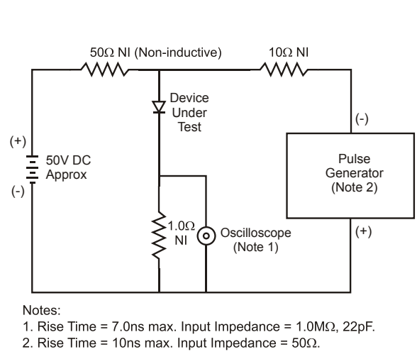
Fig. 5 Reverse Recovery Time Characteristic and Test Circuit
